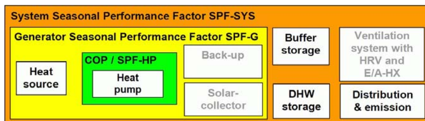
Figure 3: Definition of performance numbers and system boundaries
