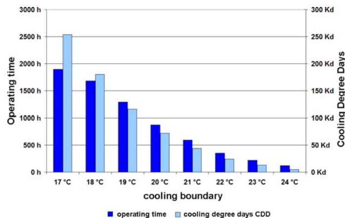
Figure 5: Typical space cooling operating times and cooling degree days
