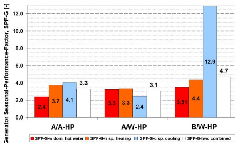
Figure 4: Juxtaposition of the generator seasonal performance numbers for the functions space heating, domestic hot water, space cooling and whole system of the three heat pump configurations A/A-HP, A/W-HP and B/W-HP
