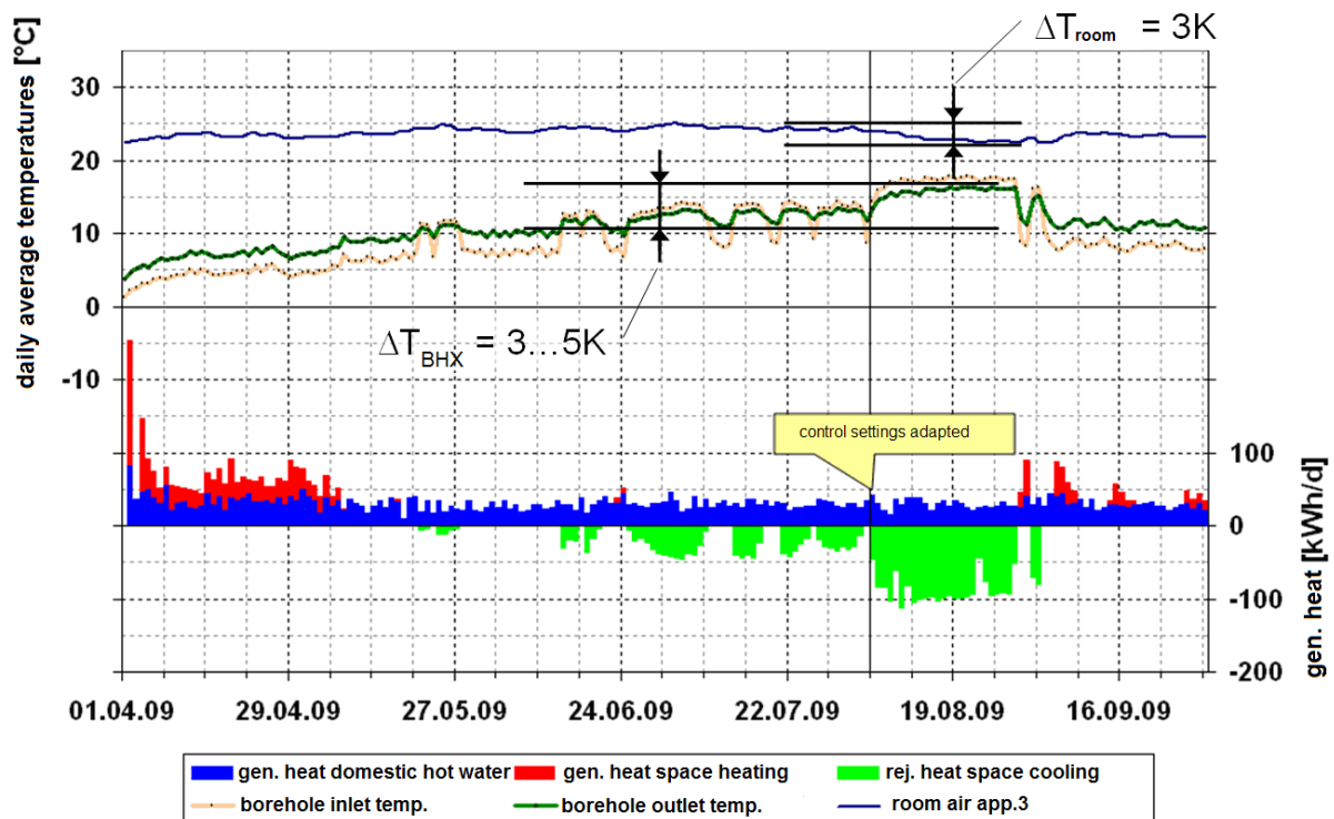
Figure 8: CosyPlace: generated heat correlated to borehole heat exchanger flow temperatures
