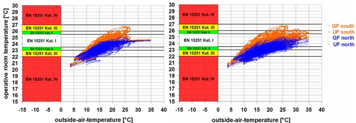
Figure 2: operative room temperature distribution correlated to the outside-air-temperature for the summer period (left: A/A-HP; right: B/W-HP)
